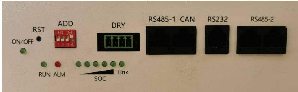
从机地址8设置示例(Example of Setting Slave Address 8)
